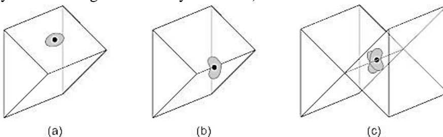
Figure(a) and (b) are 2-manifold (c) is not 2-manifold
